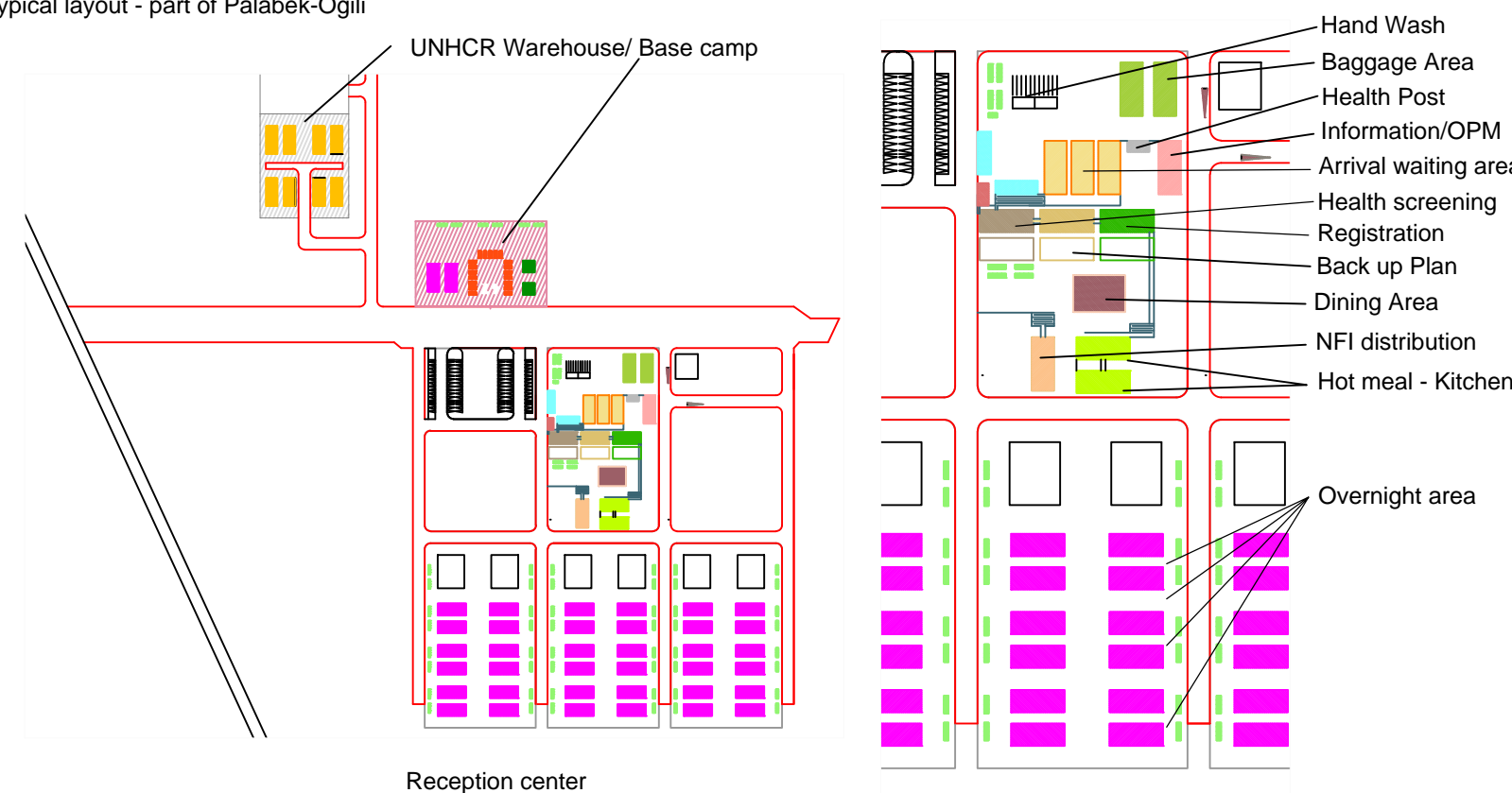
Typical layout - part of Palabek-Ogili
