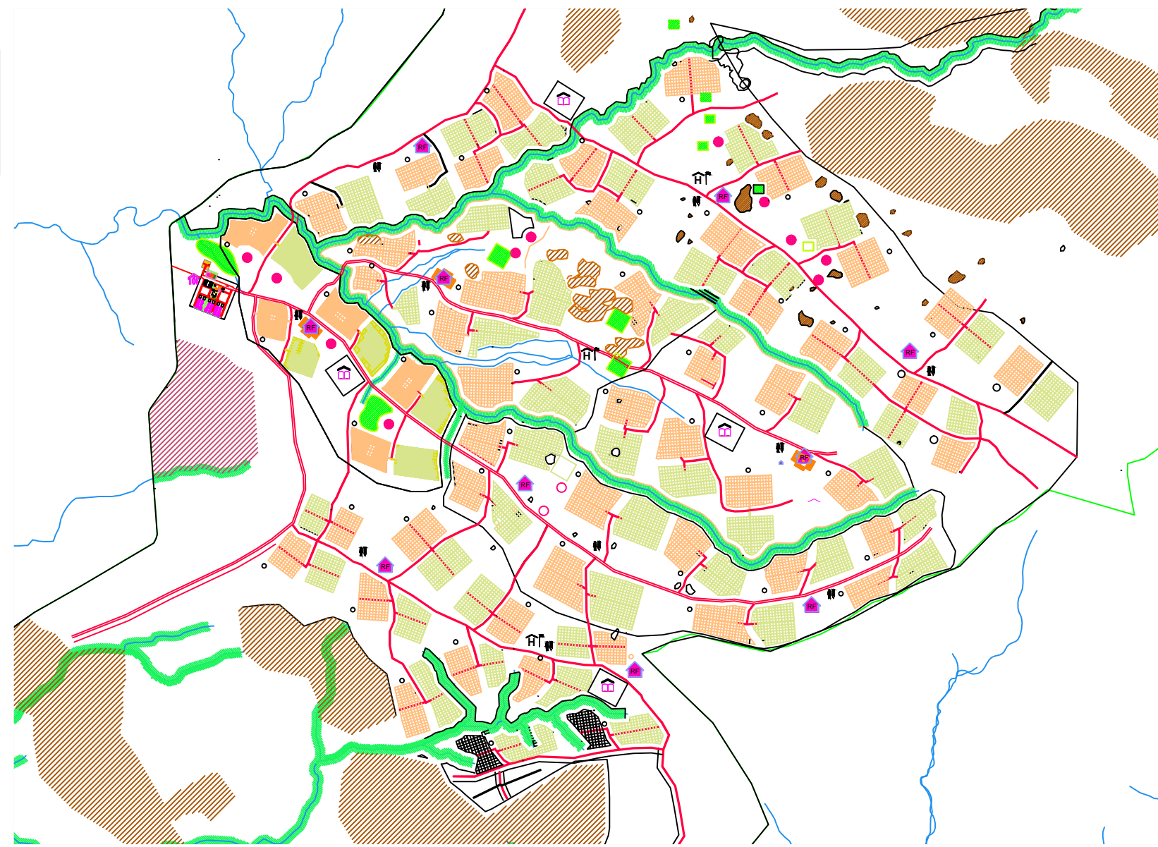
Typical layout - part of Palabek-Ogili
